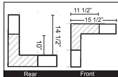
keyed corner details
